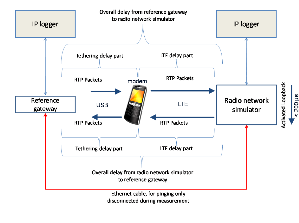
Figure C1: Measurement setup
