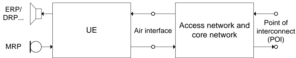
Figure 1: Interfaces (MRP, ERP/DRP..., Air interface and Point of interconnect (POI)) for specification of terminal acoustic characteristics
