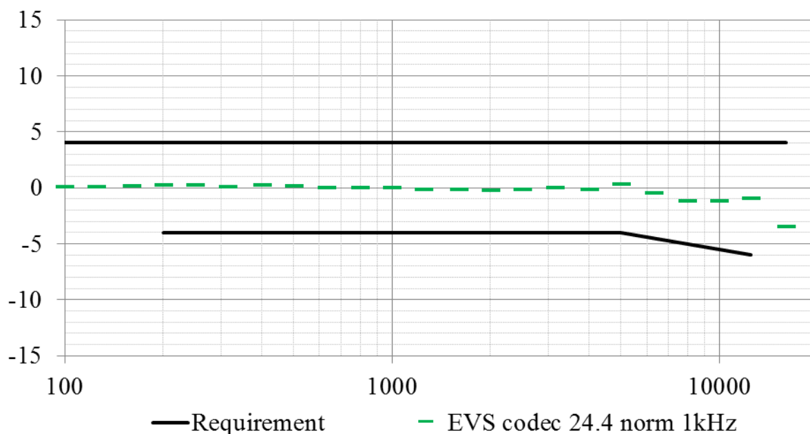
Figure 15: Handset and headset sending sensitivity/frequency masks. The frequency response of the EVS codec operating as specified in TS 26.132 (super-wideband 24,4kbit/s, using the specified P.501 speech test signal), is plotted for reference, normalized to 0dB at 1kHz.
